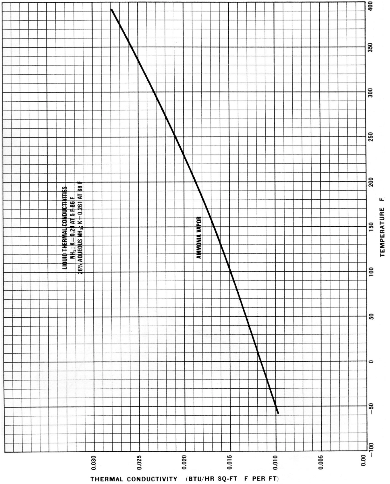
Figure 6 THERMAL CONDUCTIVITY OF AMMONIA
