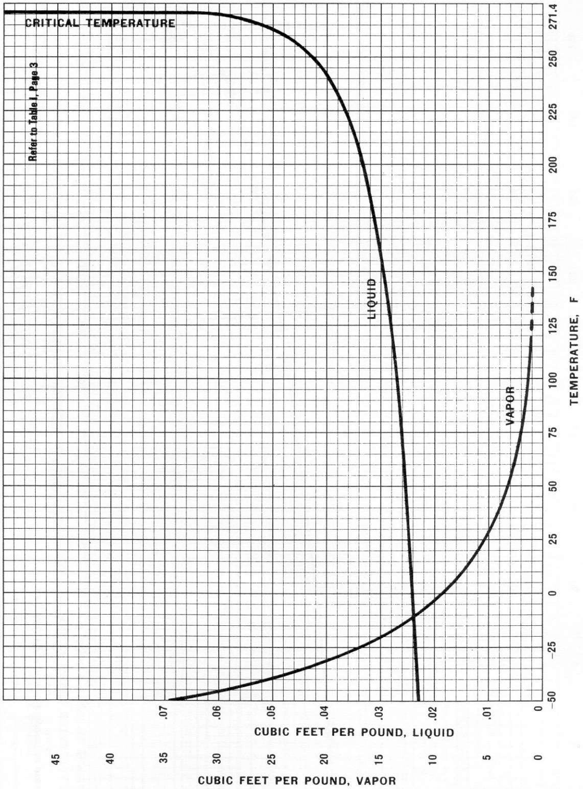
Figure 3 SPECIFIC VOLUME OF AMMONIA AS LIQUID AND VAPOR VS. TEMPERATURE
